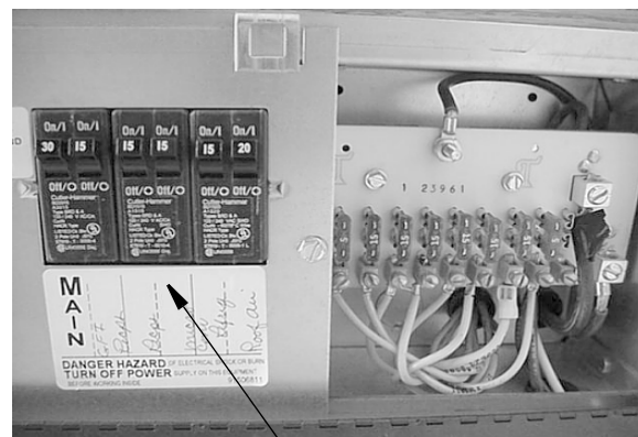
110-Volt Circuit Breakers Shown for Models 26P, 29R, 30B
