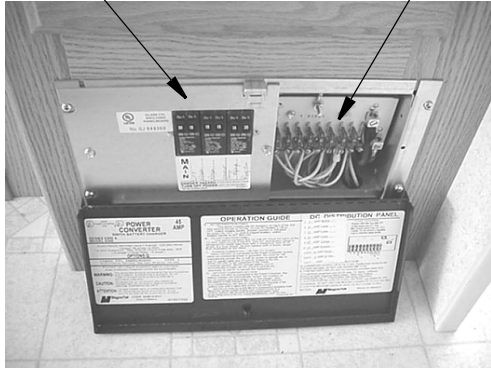
Load Center
