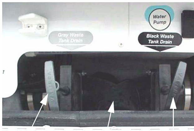
Gray Tank Dump Valve Sewer Hose Outlet Black Tank Dump Valve
