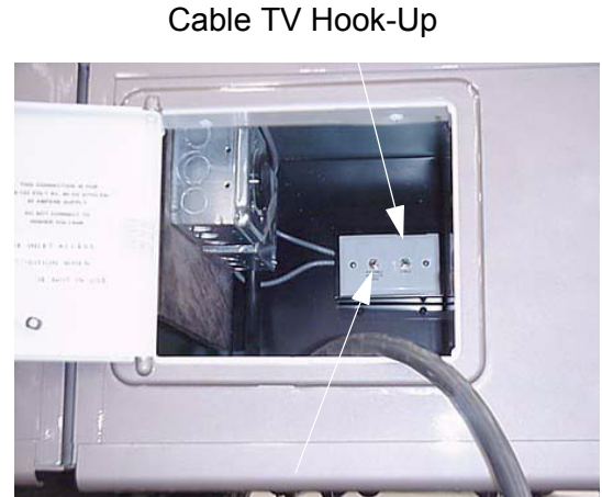
Portable Satellite Dish Hook-up in Shoreline Compartment
