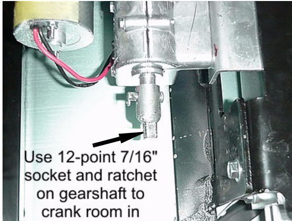
Models 26A or 29H Front Slideout Room Motor/Gear Assembly (view from ground)
