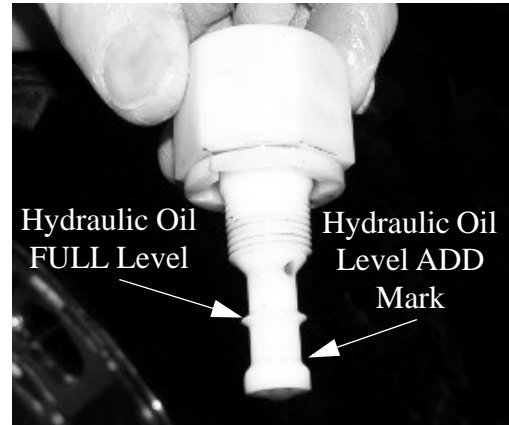
Hydraulic Oil Breather Cap/Dipstick -Typical View
