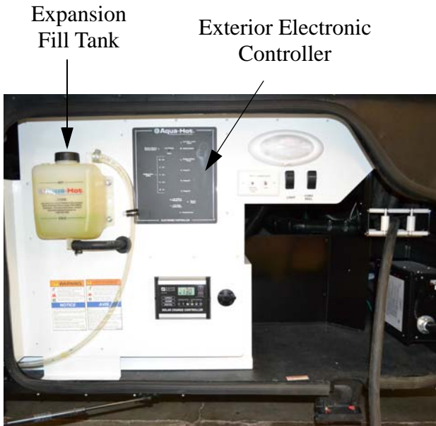
Hydronic Heating System (Located in driver side compartment) -Typical View
