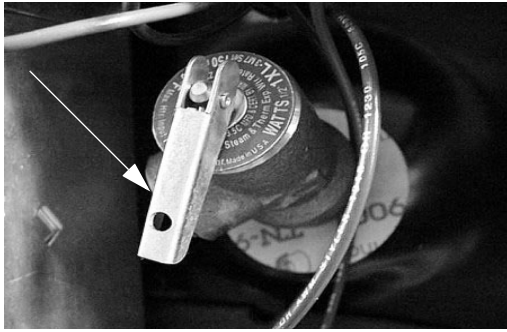
Pressure-Temperature Relief Valve (Lift handle only when water heater is cold) -Typical View
