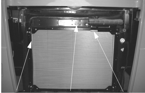
Air Filter Restriction Indicator Engine Diagnostic Connector Engine Coolant Reservoir Service Points (Shown with grille open) -Typical View
