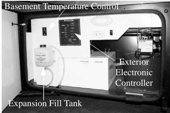
Hydronic Heating System (Located in driver side compartment behind front wheel well) -Typical View
