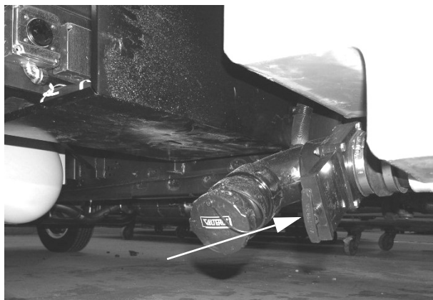
Black Waste Tank Drain Valve (Located beneath coach on mid-driver side) -Typical View
