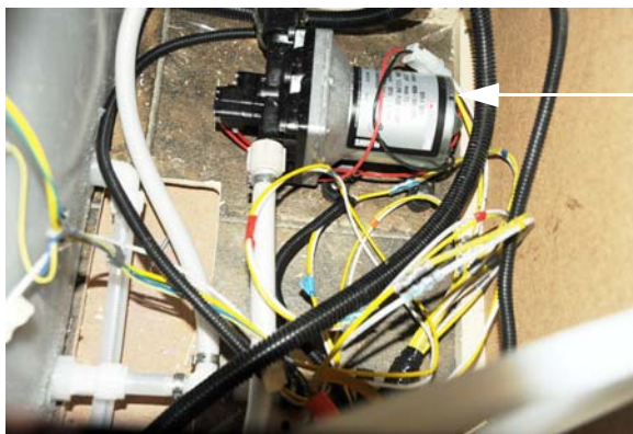
Water Pump (Located beneath bed - lift mattress to expose access hole) -Typical View
