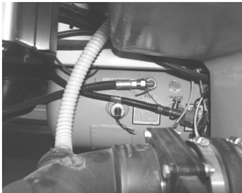
Propane Gas Tank (Located under center of coach) -Typical View
