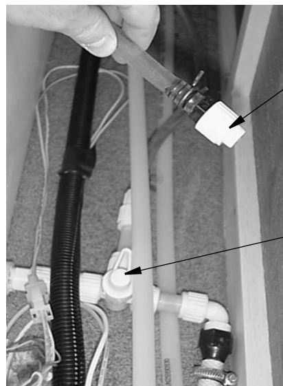
RV Antifreeze Siphon Tube and Winterization Valve
