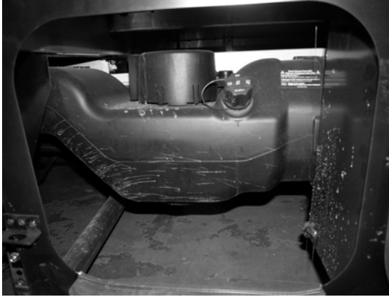
Diesel Exhaust Fluid Fill Tank (Located in passenger side compartment behind entrance door) -Typical View
