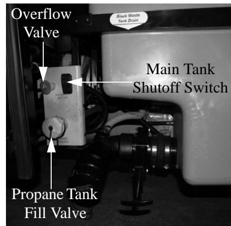
Propane Gas Access (Located in driver side compartment) -Typical View
