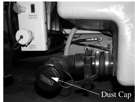
Sewage Drain Outlet (Located in driver side compartment) -Typical View
