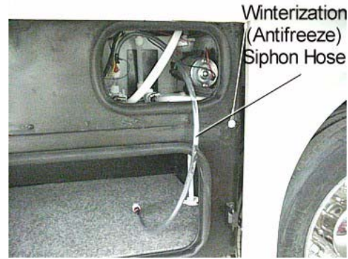
RV Antifreeze Valve -Typical Installation
