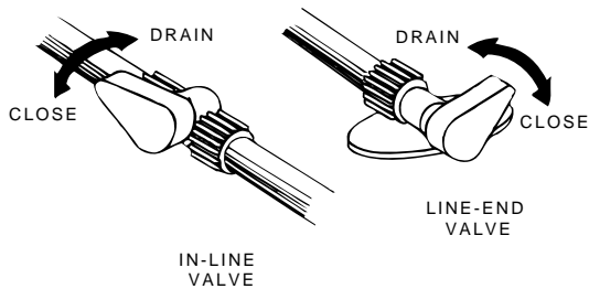
Waterline Drain Valves (Typical)
