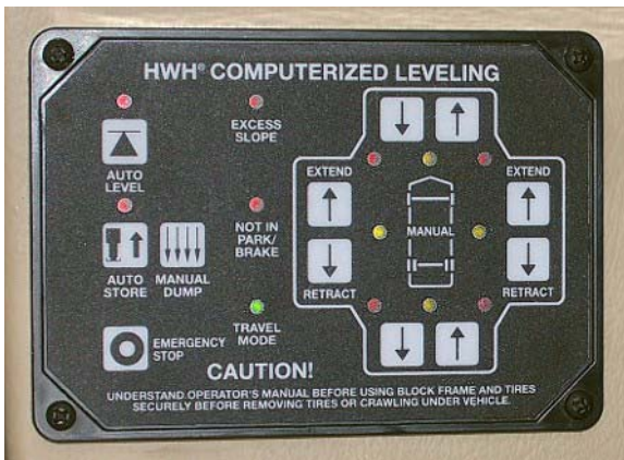
Leveling System Control Panel (Located on dash) -Typical View
