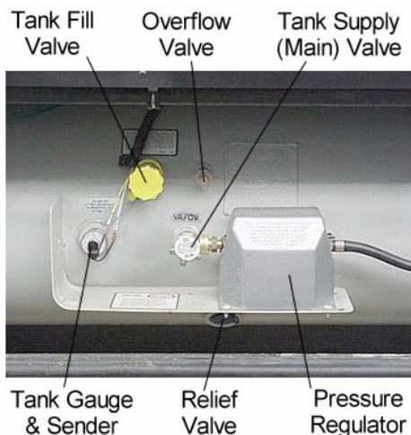
Propane Tank Features (Typical)
