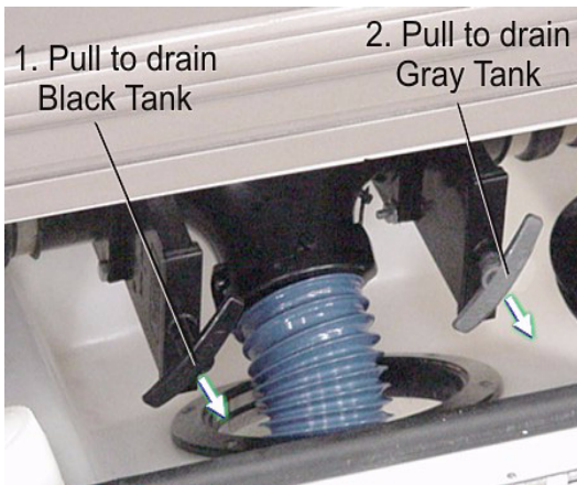
Holding Tank Dump Valves (typical)
