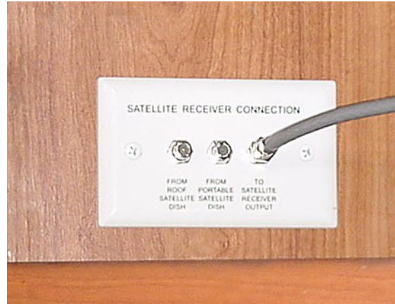
Interior Connection for Satellite Receiver
