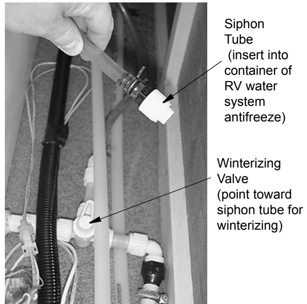
Winterization Valve (See chart at end of section for location)
