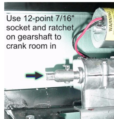
Model 327L - View of motor/gear assembly from ground
